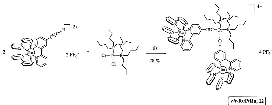
Fig. 10. Synthetic procedure followed for the preparation of cis -RuPtRu ( 12 ): (i) CuI (ca. 2 mol%), (\text{iPr})_2\text{NH} , \text{CH}_3\text{CN}/\text{THF} , 25^\circ\text{C} , 5 days.
