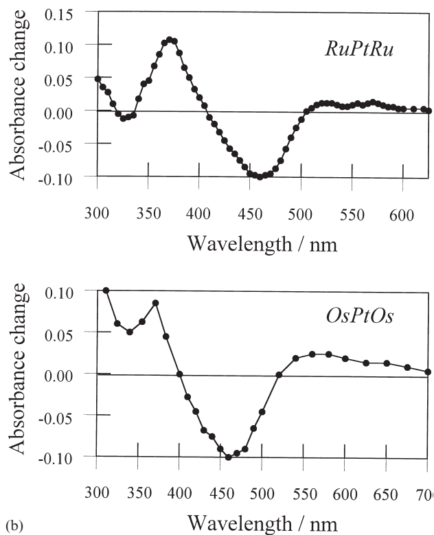
Fig. 12. (a) Luminescence and (b) differential absorption spectra recorded for the triplet excited states of trans -RuPtRu ( 6 ) and the corresponding trans -OsPtOs complex in deoxygenated acetonitrile. In each case, the spectrum closely resembles that recorded for the parent complex.
