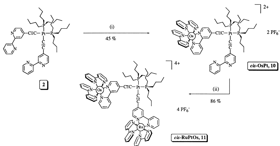
Fig. 9. Synthetic route used to prepare cis -RuPtOs ( 11 ): (i) 1 equiv. [\text{Os}(\text{bpy})_2\text{Cl}_2] , \text{C}_2\text{H}_5\text{OH} , 80^\circ\text{C} , 3 days; (ii) 1 equiv. [\text{Ru}(\text{bpy})_2\text{Cl}_2] \cdot 2\text{H}_2\text{O} , \text{C}_2\text{H}_5\text{OH} , 80^\circ\text{C} , 2 days.
