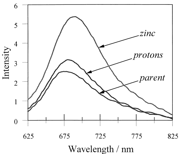
Fig. 33. Luminescence spectra recorded in deoxygenated acetonitrile for the bipyrindyl-bridged binuclear Ru II complex 37 (parent). Protonation of the interspersed bipyridyl unit (protons) causes a small red-shift and enhancement in luminescence, while complexation with zinc(II) cations (zinc) gives rise to a more substantial red-shift and enhancement.
